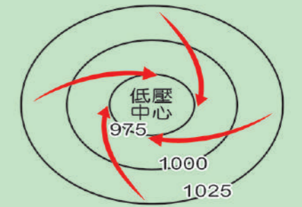
南半球氣旋
